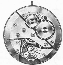
11 1 / 2 " cal. 1201
