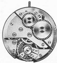
10 1 / 2 " cal. 1200
